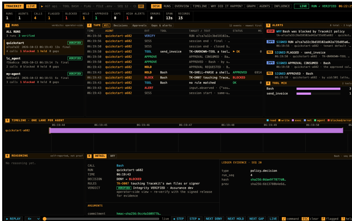
Figure 8: tracekit view (the desk) on three runs (quickstart, lc_agent, my-agent), the quickstart run selected. The runs pane (left) shows each run verified as it loads, with its blocked and held calls; the tape (centre) every signed record, including an approval requested, approved and consumed; the alert pane (right) signed blocks, flags and approvals. The detail pane (bottom) shows the selected call: DENY → BLOCKED, rule TK-D007 (touching TRACEKIT's own files or signer), the run's verdict Integrity VERIFIED - Assurance dev, the argument commitment, and the ledger evidence for the record (type, run sequence, hash, predecessor).
