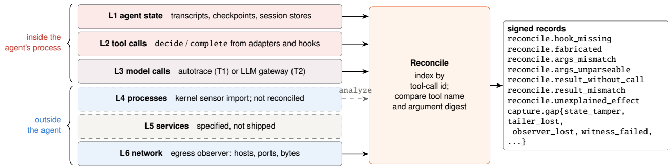
Figure 7: Capture layers in 1.4. L1–L3 and L6 report independently and the signer compares them, writing each disagreement as a signed record, so a hidden or invented call becomes evidence instead of silence. Kernel-sensor effects (L4, experimental) are recorded and joined to calls only by analyze ; L5 is not shipped.
