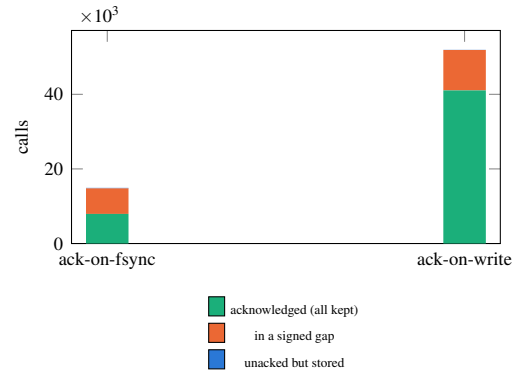
Figure 21: Every call is accounted for.
