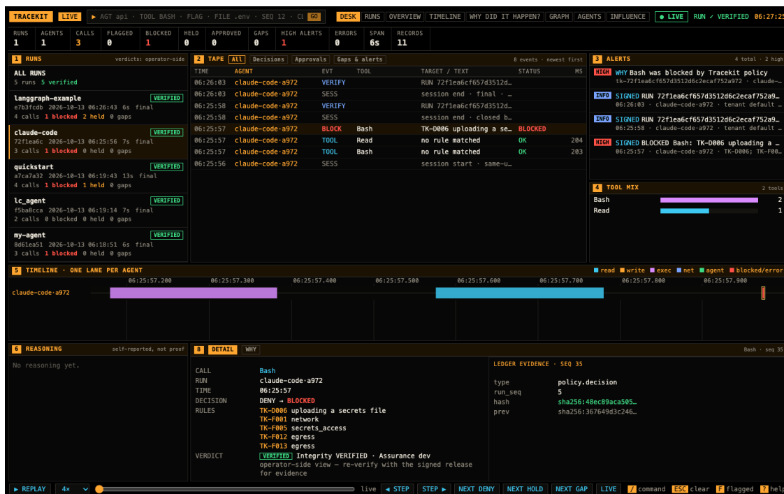
Figure 9: A Claude Code session through the v2 hook (tracekit init --dev --v2). A Bash call uploading a secrets file is denied before it runs with TK-D006; the detail pane lists the other rules it matched (network, secrets access, egress) and the run verifies.
