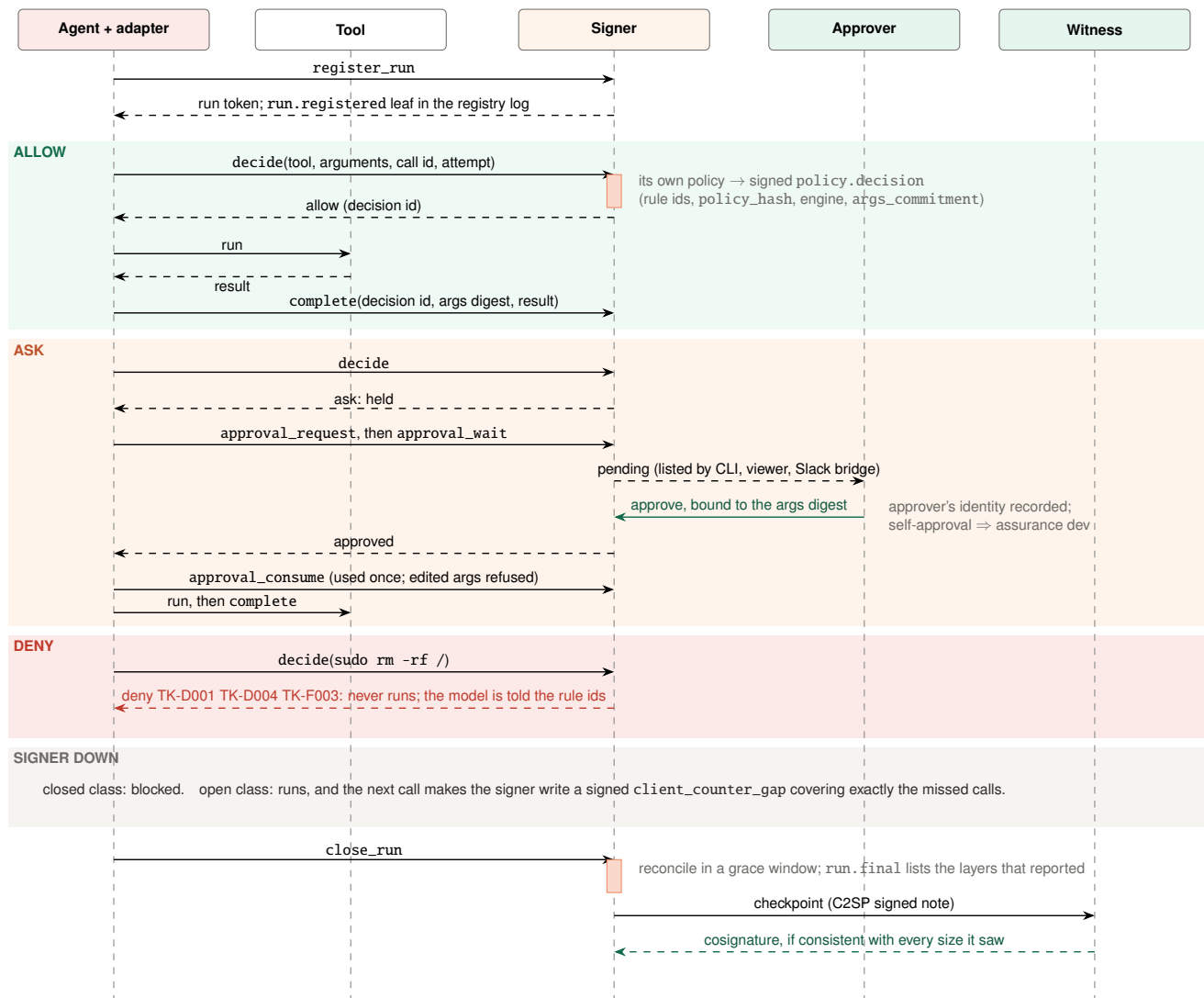
Figure 3: The life of a run. The agent only asks; every decision, approval, gap and result is written by the signer. A held call runs only after an approval bound to its exact arguments, which can be consumed once.
