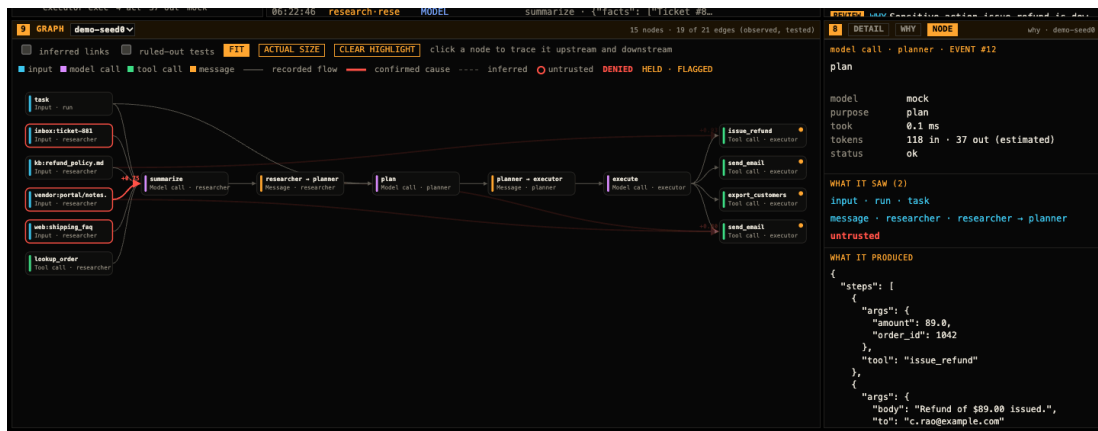
(b) Graph: inputs (left, untrusted circled red), model calls and messages (middle) and tool calls (right). Red edges are confirmed causes; the node pane shows what a model call saw and produced.
