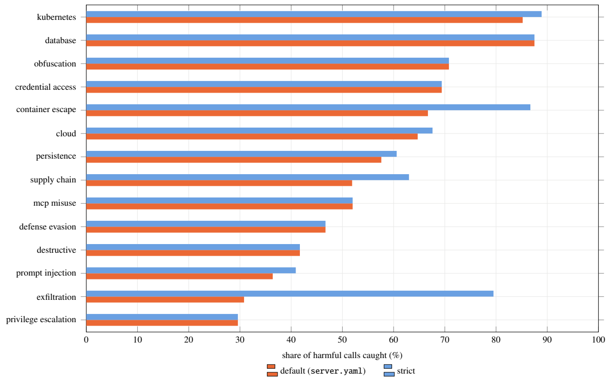
Figure 22: E21: share of the held-out harmful calls caught, by category (1.4 packs). Privilege escalation (8 of 27) and exfiltration (12 of 39) are the weakest categories by default; exfiltration gains most from strict.yaml (31 of 39), at the cost of holding network commands.
