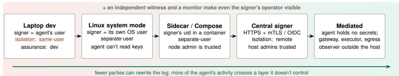
Figure 2: Deployment ladder. The agent’s code is the same at every step; the recorded isolation and the assurance a verifier can reach change.
