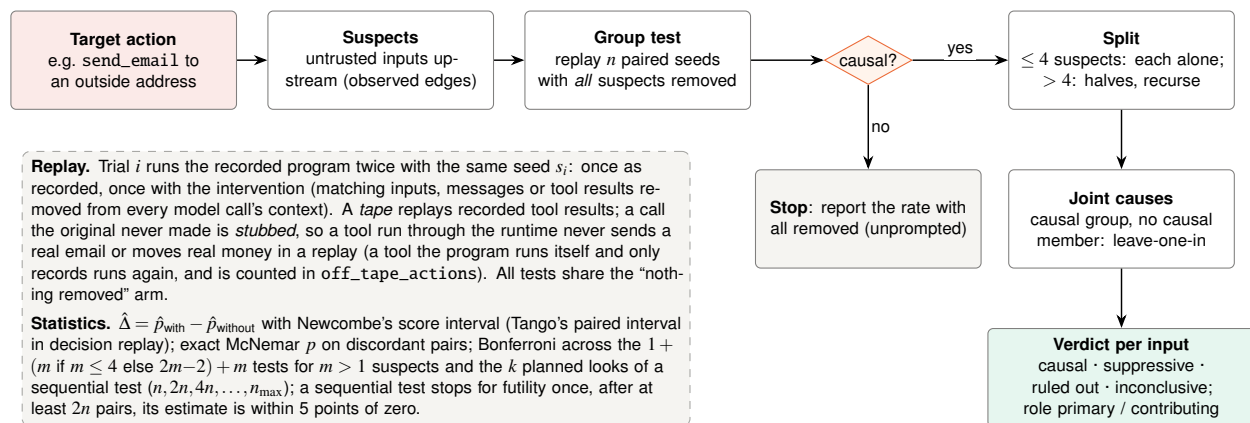
Figure 16: Attribution ( find the cause ). Replay with each suspect removed turns “reached the action” into “changed how often the action happens”, with an interval and a multiplicity-corrected verdict.
