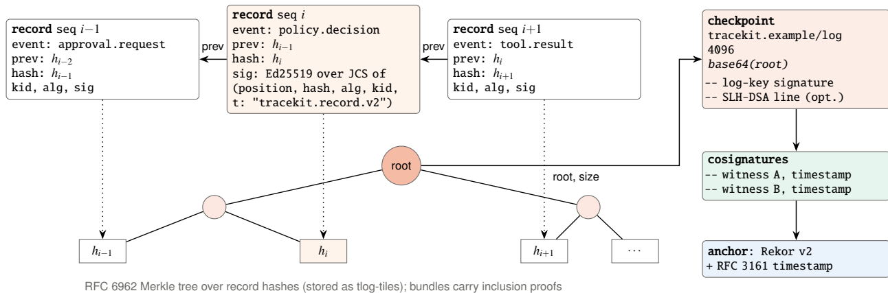
Figure 4: Records, tree and checkpoint. Each record is signed and carries the hash of the run's previous record, so a changed byte fails at that record. Record hashes are leaves of an RFC 6962 tree whose root a C2SP checkpoint signs; witnesses cosign the checkpoint only if it is consistent with every size they have seen.
