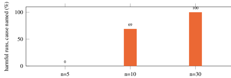
Figure 23: The replay budget has a floor (simulated model, 20 runs per scenario).
