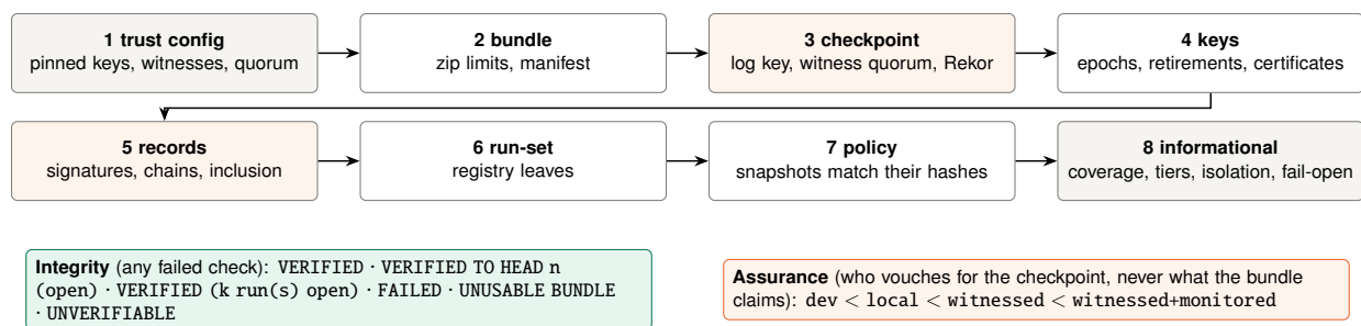
Figure 5: Verifier pipeline. Every check produces a line; any failed check line makes integrity FAILED (an unreadable trust config or bundle is UNUSABLE BUNDLE or UNVERIFIABLE). Assurance is computed separately from who vouches for the checkpoint.
