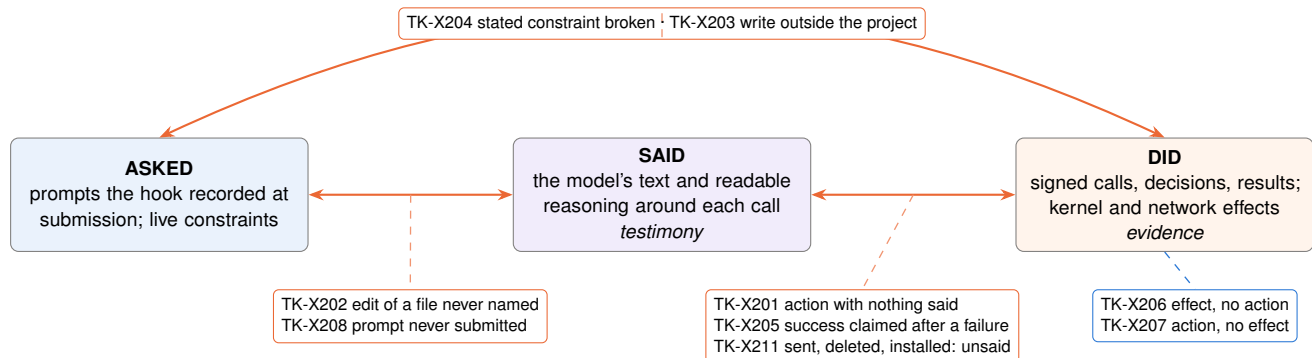
Figure 15: The three channels and the checks between them. Each finding is signed, cites the records it rests on, and never alters the integrity verdict.
