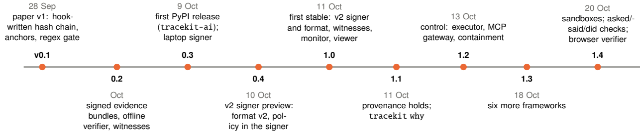
Figure 24: Release history, September to October 2026 (dates from the changelog; 1.4.1, a shell-parser hardening patch, followed on 21 October).
