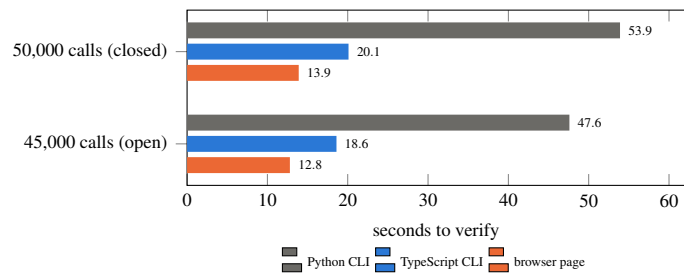
Figure 20: Verifying the largest bundles: runs of 45,000 and 50,000 calls (90,002 and 100,002 records; 24.8 and 27.6 MB zipped).
