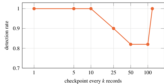
Figure 19: E1: a key holder edits one record at a random position and re-signs the rest. Records after the last checkpoint are unprotected. At k = 120 the single checkpoint is the head itself.
