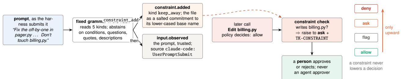
Figure 14: The life of a live constraint. The hook reads the limit from the prompt and the signer signs it before the prompt itself. A later call that breaks it is raised to ask after the policy has decided, so a constraint can only move a decision up the order on the right.
